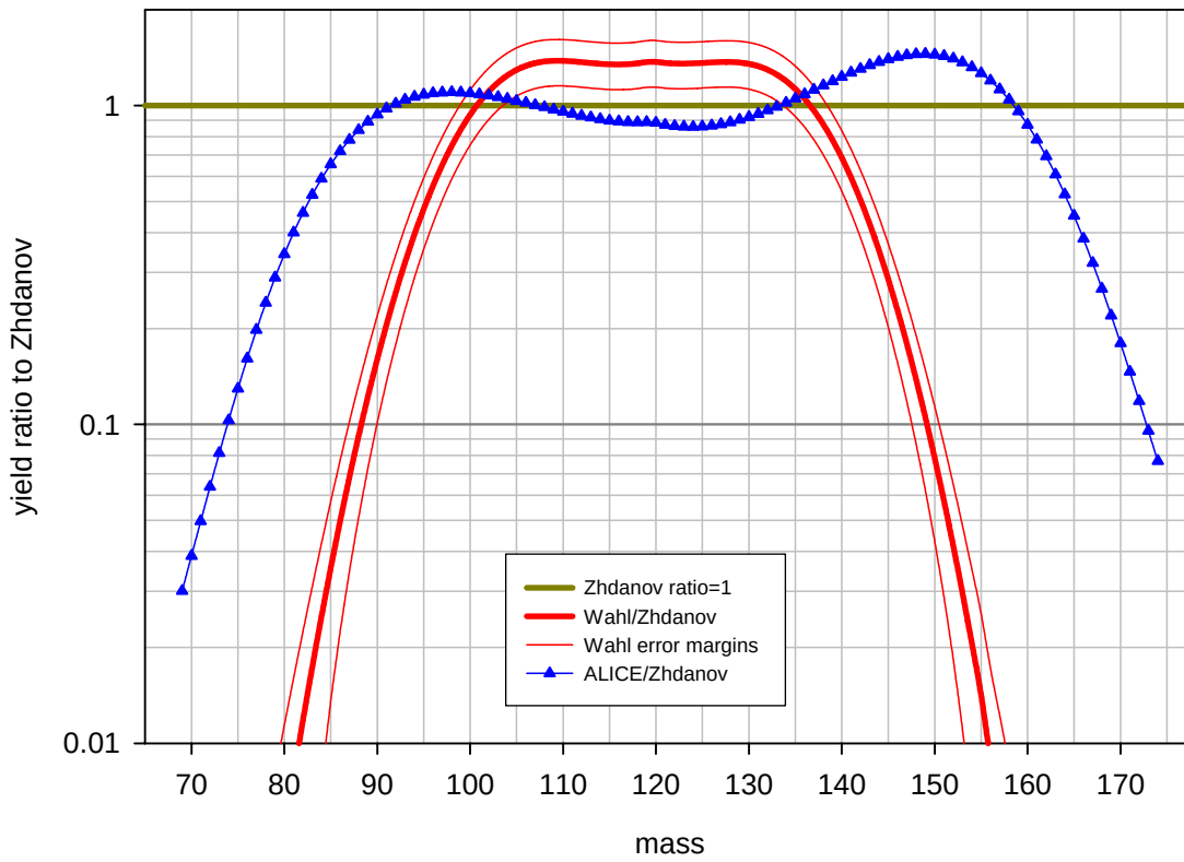
Benchmark B: ^{244}\text{Cm} at 160 MeV, pre-neutron emission yield ratio to Zhdanov's data
